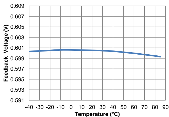
Figure 7. Feedback Voltage vs. Temperature
