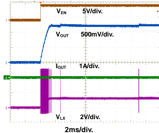
Figure 14. Power On through EN Waveform
